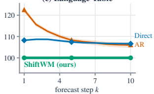
(c) Language-Table
