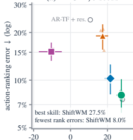
(a) DROID, 3 seeds
