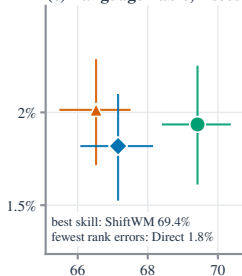
(c) Language-Table, 1 seed
