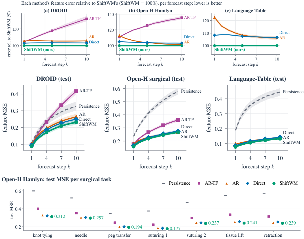
Figure 9: Forecast error per step k and per surgical task. Top: each baseline's error relative to SHIFW's (SHIFW = 100%; bands: paired 95% bootstrap). Middle: absolute feature MSE. Bottom: Hamlyn test MSE per task (mean over horizons and 1 seed(s)).
