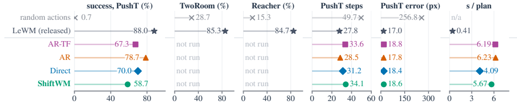
Figure 12: Closed-loop planning , official LeWM protocol (50 episodes \times 3 planner seeds). LeWM and random actions are references; matched predictors are planned on PushT only. Steps: mean to first success (budget 50); error: median final distance to the goal.
