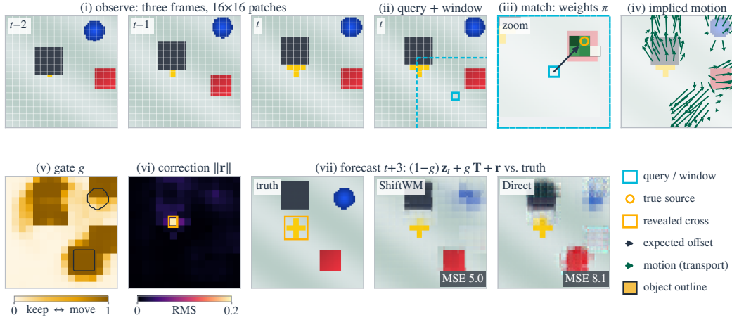
Figure 13: The mechanism on one toy window. (i) Observed frames; (ii) a query patch and its window; (iii) transport weights; (iv) motion where the gate exceeds 0.5; (v) gate; (vi) correction; (vii) forecast at t+3 .
