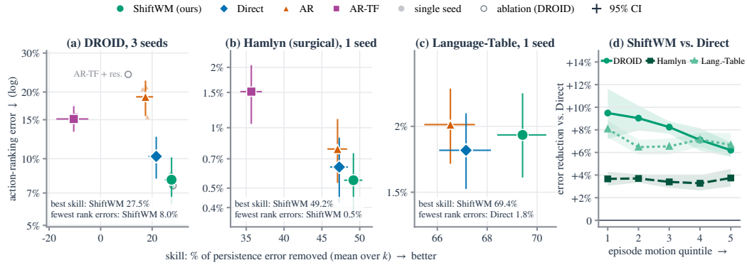
Figure 10: Forecast skill versus action ranking (test). (a–c) Lower right is better; large markers: seed means with 95% CIs; hollow: DROID ablations. (d) Error reduction of SHIFW over Direct per quintile of episode motion.
