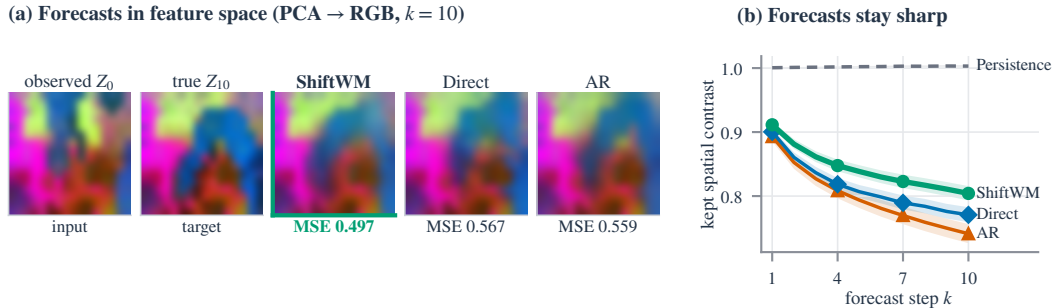
Figure 5: Forecasts in feature space. (a) Held-out forecasts at k=10 (shared PCA to colour). (b) Spatial contrast kept by each forecast, relative to the truth (95% CIs over test episodes).
