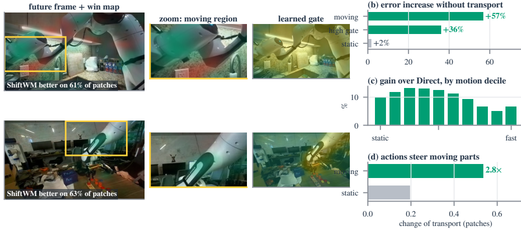
(a) Where ShiftWM beats Direct on held-out DROID (green: lower error)
