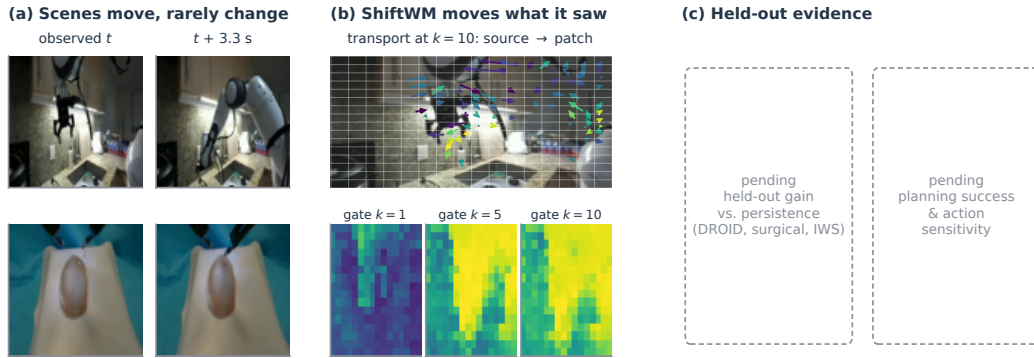
Figure 1: SHIFTWM forecasts by moving what it has already seen. (a) In real robot video (DROID, top) and surgical robot video (OpenH, bottom), the scene 3.3 s later mostly contains the same content in new places. (b) SHIFTWM predicts each future patch by transporting observed features along a learned field. Arrows run from the expected source location to the predicted patch on a held-out DROID episode, and the gate maps show that transport is used more at longer horizons and around the moving arm. (c) Held-out gains over persistence across robot, surgical and single-image benchmarks, together with planning success and action sensitivity (Sections 4 and 5).
