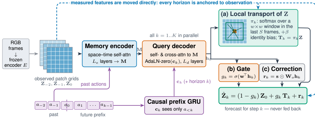
Figure 2: SHIFTWm architecture. A frozen encoder maps the H observed frames to patch grids \mathbf{Z}_{-H+1:0} . The memory encoder mixes them over space and time. For each future step k , a decoder conditioned on the causal action-prefix state \mathbf{c}_k produces per-patch hidden states \mathbf{h}_k . The output combines three terms: (a) local soft transport of observed features, (b) a gate between the identity path and transport, and (c) a scaled correction. Every horizon reads measured features directly, so no forecast is fed back as input.
