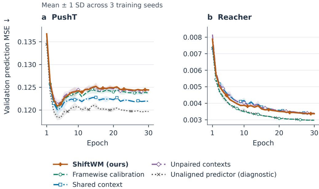
Figure 14: Validation prediction loss over the completed training campaign. Curves and shaded bands show means and sample standard deviations over three training seeds at common logged epochs. Colors and line styles identify model variants. No future epochs are extrapolated, and bands are not confidence intervals. The two panels have separate vertical scales. These are validation records, not test-set or planning-performance results.
