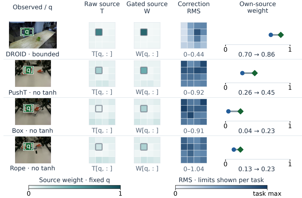
Figure 7: A measured decoder view: read, retain and correct. Each row uses the middle-ranked trajectory’s fixed window (DROID: 71st of 141; IWS: fifth of ten, in decreasing-gain order). DROID uses bounded ShiftWM; reserved IWS uses its no-tanh ablation. Weights and corrections are at DROID h = 10 and IWS offset 59 ( H = 60 ). The outlined coordinate q is always row 2, column 2 of the feature grid, not an object localization. Maps T[q, :] and W[q, :] show all 16 observed-source weights for that destination patch, averaged over three seeds on a common [0, 1] scale. Right: the same-location weight before (circle) and after (diamond) gating. This increase follows algebraically from W = I - D + DT and does not establish an accuracy gain. Correction maps show the mean of per-seed channel RMS values, with separate task scales printed below. These are feature-mixing diagnostics, not semantic attention or physical motion. Recorded scenes: DROID (CC BY 4.0) and RLA-WM/IWS.
