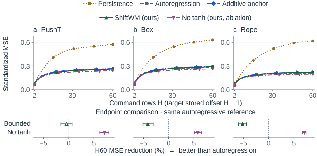
Figure 8: Single-observation transfer: forecasting and the effect of the correction bound. Top: all five predictors and all 59 future offsets on recorded IWS tasks; H counts native command rows and predicts stored offset H - 1 . Bottom: H = 60 MSE reduction versus the same autoregressive baseline; right is better and bars are paired 95% intervals. The bounded model has no consistent advantage here; removing only tanh improves all three endpoint means. Means weight trajectories and three seeds equally. The original 27-model study and nine-model follow-up are development comparisons; the latter is exploratory. Table 14 gives every plotted contrast and the original primary comparison; Table 15 retains all four metrics. Reserved evaluation is excluded.
