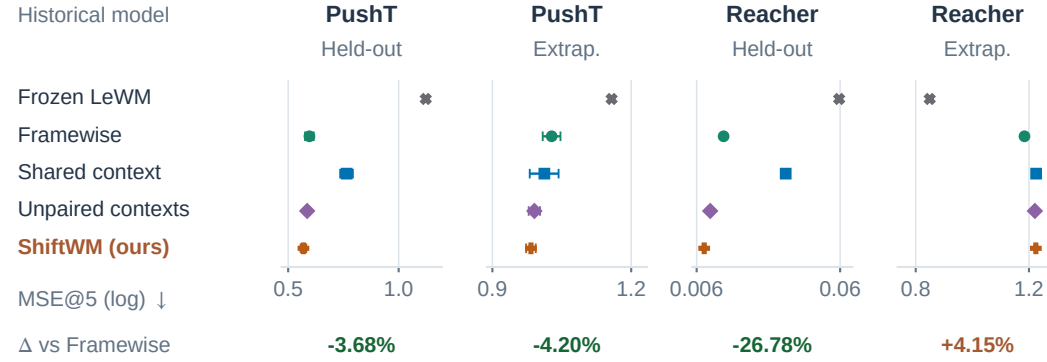
Figure 13: Historical context model: complete forecast comparison. Each panel retains all five aligned methods. Points and bars show means and sample SD across three training seeds; Frozen LeWM has one checkpoint and no seed SD. The target is fixed-reference latent MSE after five recursive blocks (25 native actions), using recorded future actions. Axes are logarithmic with panel-specific limits; latent coordinates differ between environments. The last row is the signed relative MSE change of ShiftWM (ours) versus Framewise: negative is better, with no interval or significance inference. Reacher extrapolation is unfavorable, and Frozen LeWM has its lowest mean. The unaligned diagnostic remains in the complete table, outside this aligned comparison. These are forecasting results for the earlier model, not closed-loop success or evaluation of the newer spatial architecture.
