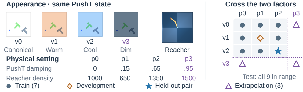
Figure 12: Crossed appearance and dynamics in the historical simulation study. Full recorded simulator frames illustrate PushT and Reacher. The four PushT views apply the exact RGB transforms to one state; physical settings change damping or arm and finger density together. Training and ordinary validation use seven pairs; (v_1, p_1) is development and (v_2, p_2) is held-out composition. Three additional pairs use new factor values; blank cells are unevaluated. Independent test trajectories cover all nine in-range pairs, including familiar combinations. Trajectory seeds are split before paired rendering; factor IDs are unavailable to the deployed model. This is the historical context-model protocol.
