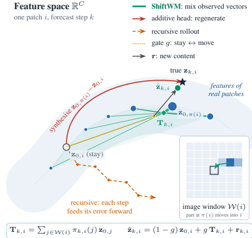
Figure 3: One patch in feature space. SHIFTWM mixes observed vectors; additive heads regenerate the displacement; recursion feeds drifts.
