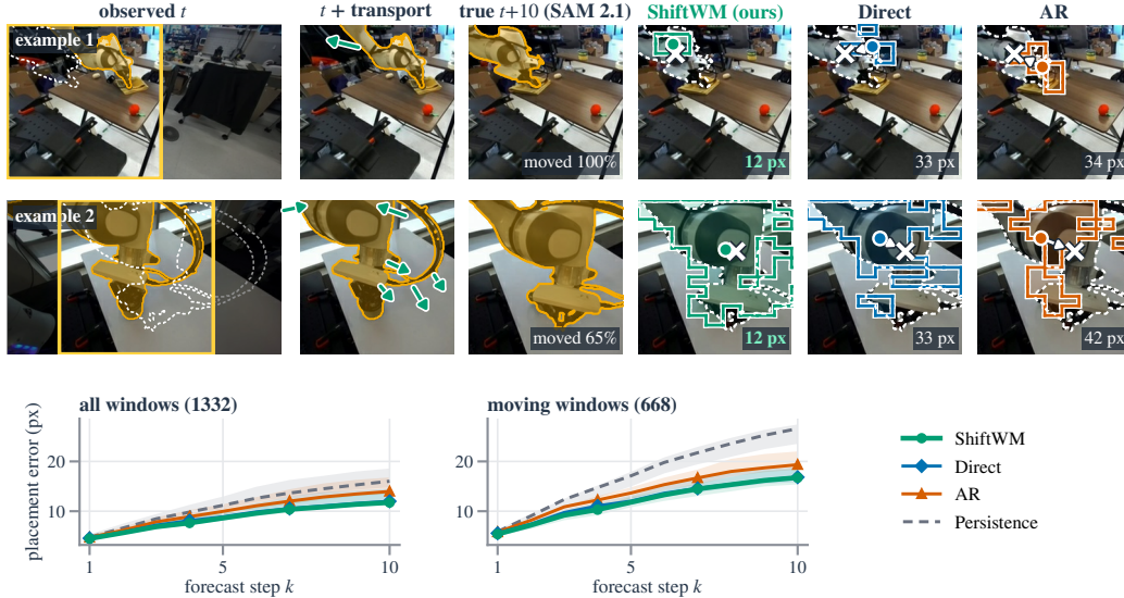
Figure 15: Arm placement, DROID (target: robot arm; 1332 windows, 123 episodes). All method columns show the same true frame t+10 . Examples: the two moving windows (distinct episodes) with the largest k=10 placement advantage of SHIFTWM over the better baseline, among windows where SHIFTWM’s error is below its median; illustrative, averages in Table 19. Bottom: placement error vs. horizon (95% CIs over episodes). Columns as in Figure 14.
