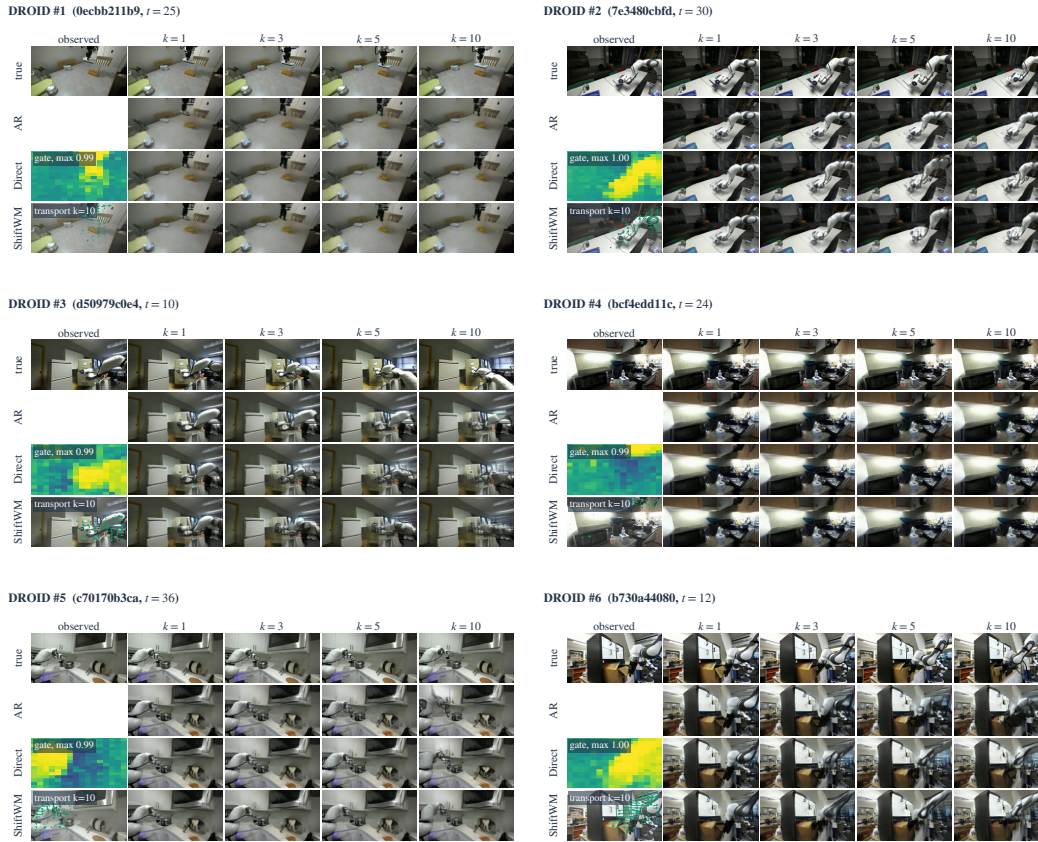
Figure 17: DROID test rollouts (random selection).
