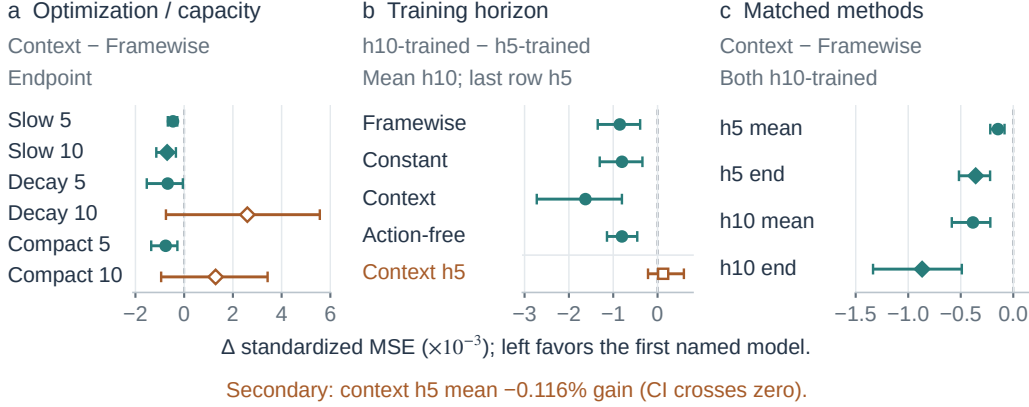
Figure 9: Optimization, capacity and horizon controls for the historical context model (ours), on original DROID validation. Context denotes the factorized two-context model; Constant denotes Constant dynamics. (a) Context minus matched Framewise endpoint MSE under Slow, Decay and Compact interventions, at five or ten action blocks. All 36 runs train 30 epochs and use the common five-query selection objective; Compact changes predictor and context capacity jointly. (b) Ten-query-trained minus original five-query-trained mean MSE on identical ten-query-eligible windows, for every method. The separated final row retains the unfavorable matched-five-query Context secondary result (−0.116% relative gain). Training and selection horizons change together. (c) Context minus equally ten-query-trained Framewise on standard populations. Mean averages query errors; end denotes the endpoint. All 12 horizon-study runs train 30 epochs; every selected checkpoint is epoch 1. Bars are paired 95% session/seed bootstrap intervals (10,000 draws); open marks include zero. Axes use different limits but the same MSE unit. Windows are averaged within 141 episodes from 59 sessions and then three seeds equally. Standard h5 uses 1,772 windows; h10 and matched h5 prefixes use 1,631. All four-method absolute errors remain in Tables 16, 21 and 22; all 20 registered horizon contrasts remain in the tables and companion ledger. These exploratory, multiplicity-unadjusted comparisons provide no independent-test claim.
