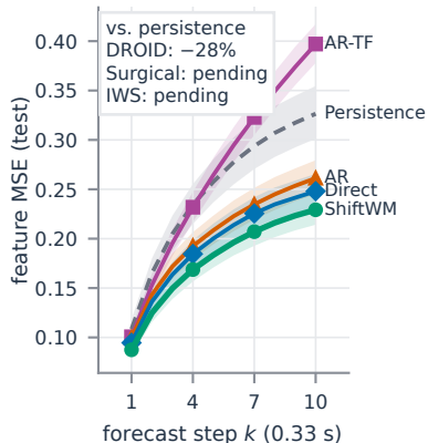
(c) Errors don't compound
