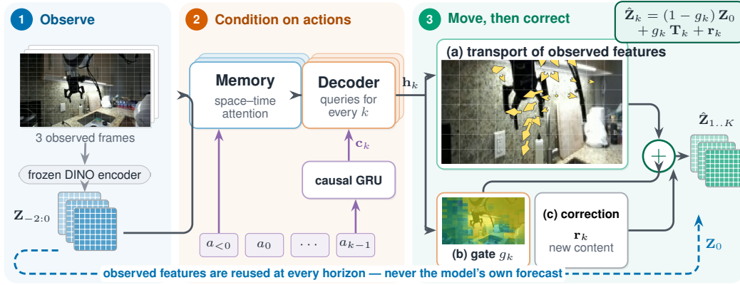
Figure 2: SHIFWWM architecture. For each horizon k , an action-conditioned decoder predicts where every patch comes from (a), whether it moves (b), and a correction (c). Insets are learned outputs on a held-out DROID episode.
