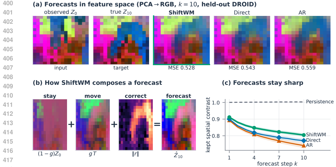
Figure 5: Inside SHIFTWM. (a) Held-out forecasts at k=10 in feature space. (b) The forecast is the sum of a kept, a moved and a corrected term. (c) Transport keeps more spatial contrast than regression (95% CIs).
