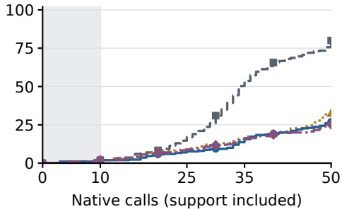
Reacher
