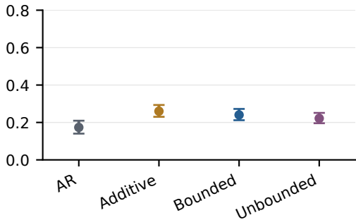
Reacher
