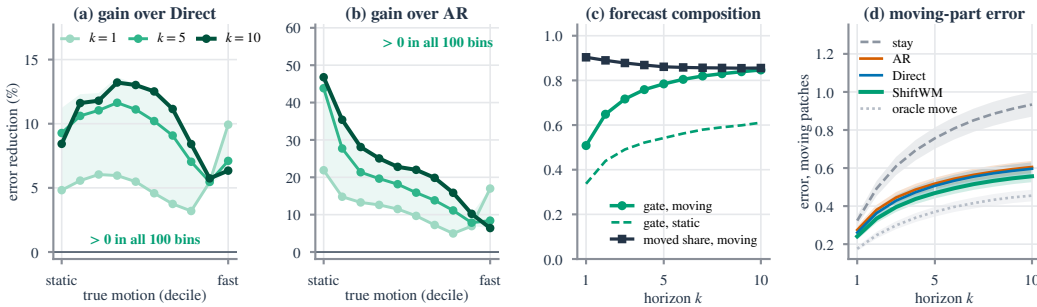
Figure 12: Anatomy of the gains (held-out DROID) . (a,b) Error reduction vs. motion decile at k \in \{1, 5, 10\} (band: all horizons). (c) Gate and share of the forecast carried by moved features. (d) Moving-part error with 95% CIs.
