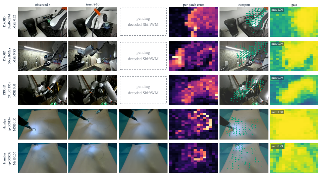
Figure 16: Failure cases.
