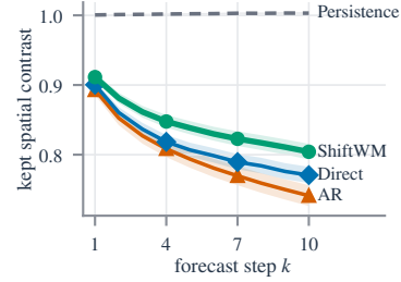
Figure 6: Forecasts in feature space. (a) Held-out forecasts at k=10 (shared PCA to colour). (b) Spatial contrast kept by each forecast, relative to the truth (95% CIs over test episodes).
