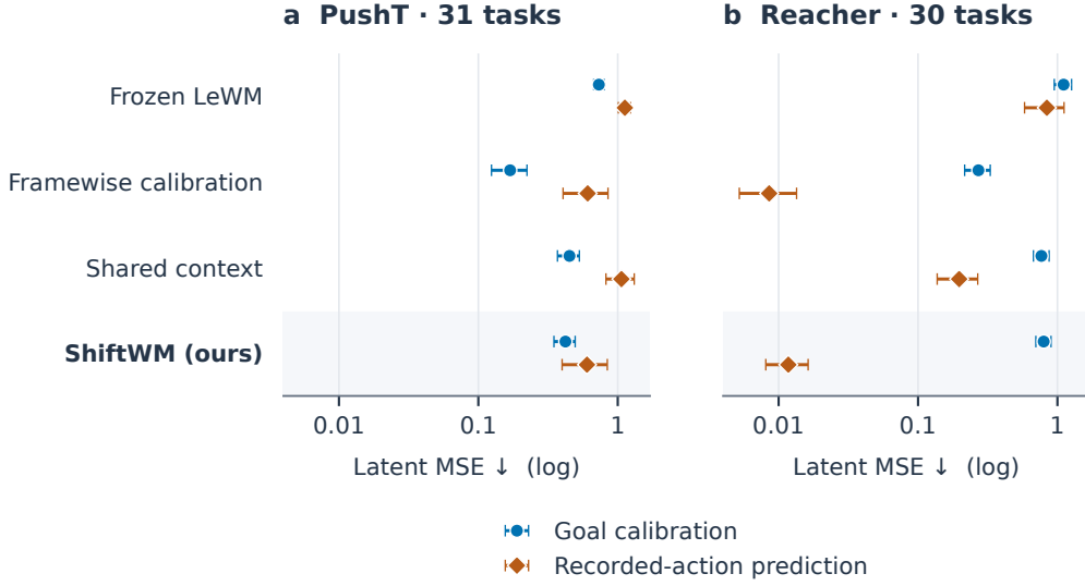
Figure 26: Prediction and goal calibration are distinct errors. Posthoc development diagnostics for frozen LeWM and three seed-0 trained models. Both errors are per-dimension MSE in fixed pre-trained coordinates against the same canonical goal; lower is better. Blue circles denote goal calibration; orange diamonds use the five recorded future action blocks. Horizontal axes are logarithmic so small errors remain visible. Error bars are 95% trajectory-seed bootstrap intervals, excluding common support-only successes; they do not measure training-seed variation. Small recorded-action prediction error alone does not establish accurate goal calibration or successful planning.
