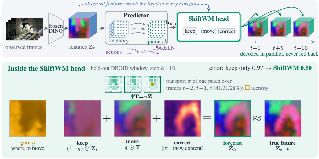
Figure 2: SHIFTWM architecture. Top: an action-conditioned predictor produces one query per patch and step; observed features reach the head directly. Bottom: on a held-out window, the forecast is the sum of kept, moved and corrected observed features.
