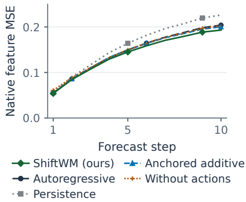
Figure 4: Candidate 4: 5.5 by 2.60 inches. ShiftWM (ours) on original DROID validation. (a) Mean endpoint feature error; each forecast step consumes five native commands. (b) Paired error reductions against autoregression, anchored additive prediction and the action-free ablation at steps 5 and 10. Error bars are 95% session/seed bootstrap intervals; connecting lines guide the eye. All 21 trained models completed 30 epochs. Other ablations remain in Table 1 and the appendix, including inconclusive context/bounding effects and unfavorable outcomes. The complete 36-contrast record remains unchanged; this is development evidence.
