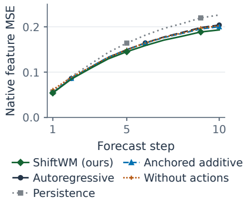
Figure 5: Candidate 5 (recommended main figure): 5.5 by 2.60 inches. ShiftWM (ours) on original DROID validation. (a) Mean endpoint feature error; each forecast step consumes five native commands. (b) Paired error reductions against autoregression, anchored additive prediction and the action-free ablation at steps 5 and 10. Error bars are 95% session/seed bootstrap intervals; connecting lines guide the eye. All 21 trained models completed 30 epochs. Other ablations remain in Table 1 and the appendix, including inconclusive context/bounding effects and unfavorable outcomes. The complete 36-contrast record remains unchanged; this is development evidence.
