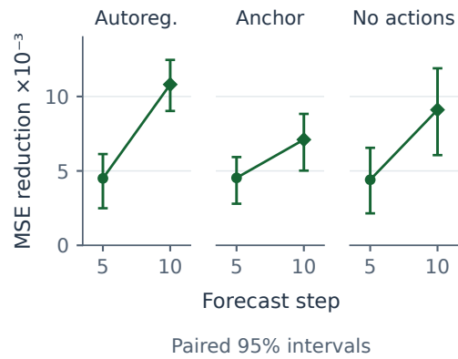
(b) ShiftWM gains vs controls
