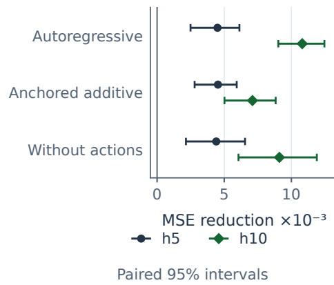
Figure 4: Candidate 4: 5.5 by 2.60 inches. ShiftWM (ours) on original DROID validation. (a) Mean endpoint feature error; each forecast step consumes five native commands. (b) Paired error reductions against autoregression, anchored additive prediction and the action-free ablation at steps 5 and 10. Error bars are 95% session/seed bootstrap intervals; connecting lines guide the eye. All 21 trained models completed 30 epochs. Other ablations remain in Table 1 and the appendix, including inconclusive context/bounding effects and unfavorable outcomes. The complete 36-contrast record remains unchanged; this is development evidence.
