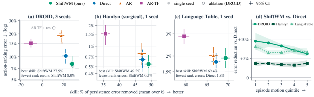
Figure 10: Forecast skill versus action ranking (test) . (a–c) Lower right is better; large markers: seed means with 95% CIs; hollow: DROID ablations. (d) Error reduction of SHIFTWm over Direct per quintile of episode motion.
