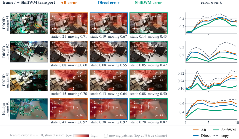
Figure 14: Largest-margin test windows. DROID and Hamlyn windows (top half of motion) with the largest k=10 gain of SHIFTWm over the better of Direct and AR. Error maps share one scale (dashed: moving patches).
