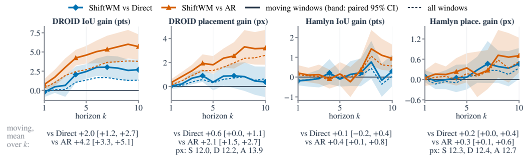
Figure 13: Segmentation read out of the forecasts. Paired gain of SHIFTWM over Direct and AR per horizon: IoU (points) and placement error removed (px of the displayed frame); bands: paired 95% CIs on moving windows. Below: moving-window means over k with CIs, and mean placement error of SHIFTWM (S), Direct (D) and AR (A).
