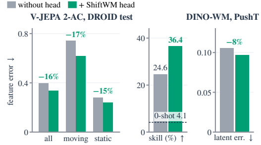
Figure 5: SHIFTWM as a plug-in head. Same model, data, schedule and loss with and without the head. V-JEPA 2-AC: DROID test, 2 seeds (dashed: released model, zero-shot); DINO-WM: PushT validation.
