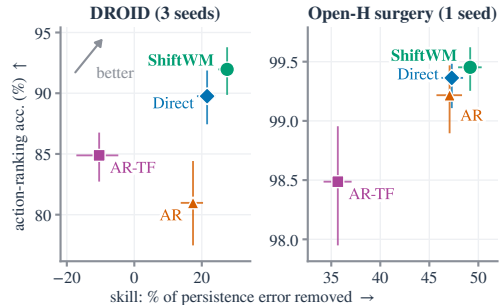
Figure 4: Better forecasts without weaker action sensitivity. Skill vs. action-ranking accuracy (95% CIs); SHIFTWM is highest on both axes on DROID and Open-H.
