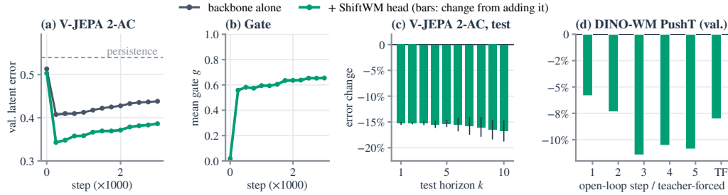
Figure 11: Plug-in heads during and after training , same data, schedule and loss with and without the head. (a) V-JEPA 2-AC validation latent error (2 seeds; band: range). (b) Mean gate of its head. (c) Change of test error per horizon (whiskers: all seed pairings). (d) DINO-WM on PushT (1 seed): change of validation latent error per open-loop step and teacher-forced (TF).
