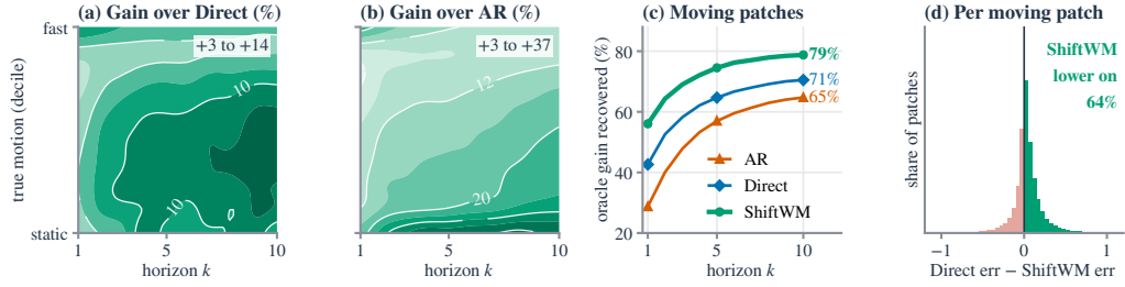
Figure 12: Where the gains lie (held-out DROID). (a,b) Error reduction of SHIFTWM per horizon and decile of true patch change (%). (c) Share of the oracle-move gain recovered on moving patches. (d) Per-patch error difference to Direct at k=10 on moving patches (green: SHIFTWM lower).
