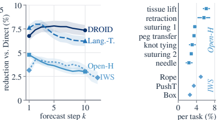
(f) Holds at every horizon and task
