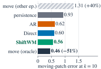
(f) Holds at every horizon and task
