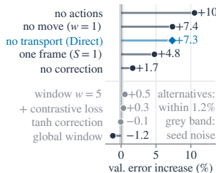
(e) Each core component matters
