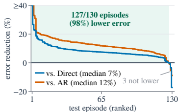
(a) Lower error on 127 of 130 episodes
