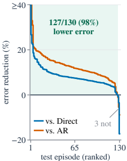
(a) Lower error, 127/130 ep.
