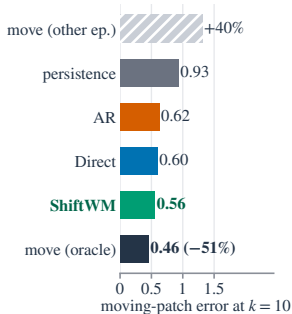
(b) Future = present, moved
