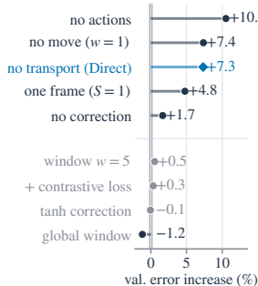
(c) Each component matters
