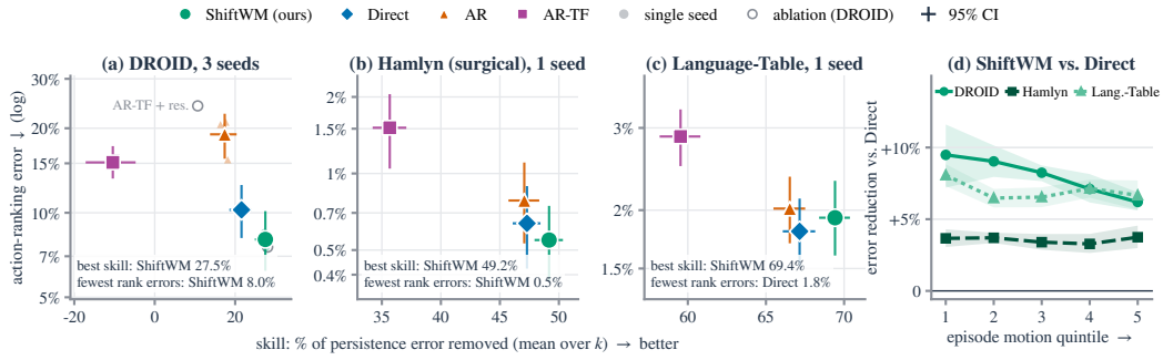
Figure 11: Forecast skill versus action ranking (test) . (a–c) Lower right is better; large markers: seed means with 95% CIs; hollow: DROID ablations. (d) Error reduction of SHIFTWM over Direct per quintile of episode motion.
