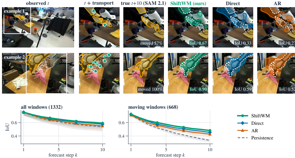
Figure 15: Segmentation view, DROID (target: robot arm; 1332 windows, 123 episodes). Examples: the two moving windows (distinct episodes) with the largest k=10 IoU advantage of SHIFTWm over the better baseline, SHIFTWm IoU \geq 0.5 ; illustrative, averages in Table 17. Columns as in Figure 14.
