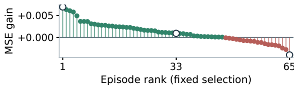
Figure 9: Residual calibration on actual DROID recordings. (a) One train-fitted scalar contracts each forecast displacement about the last observation; the schematic uses seed 0's \alpha = 0.908 . The base rollout is unchanged. (b–d) Episodes are selected by their three-seed, episode-average h5 gains: largest improvement, median and largest regression among all 65 fresh recordings. Photographs are recorded support/target frames from each first eligible window (native indices 10 and 35). Curves show that window's five measured feature errors, averaged over three seeds; vertical ranges differ between cases. Positive \Delta favors calibrated ShiftWM over equally calibrated Framewise. *The median episode improves overall but regresses in the displayed window. (e) All episode gains and regressions are shown. The separate population interval is the original paired session/seed bootstrap: MSE gain 0.001103, 95% CI [0.000290, 0.002145], or 0.742% lower mean h5 error. This measures observational forecasting, not physical control.
