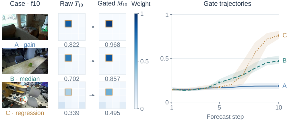
Figure 6: Measured anchoring and gate trajectories. A/B/C are the largest-gain, median and largest-regression episodes; each diagnostic uses its first eligible window, as in Figure 4. At target patch j = 5 (row 2, column 2), maps show raw source weights T_{10}[j, :] and effective weights M_{10}[j, :] . M_h = (1 - g_h)I + g_h T_h is computed within each seed before averaging. All six maps share a linear [0, 1] scale; the amber outline and numbers identify the own-source weight. Gate curves show three-seed means and min–max ranges, not confidence intervals; each forecast step uses five native commands. Full images are recorded f10 observations (DROID, CC BY 4.0). These latent-feature diagnostics do not establish physical correspondence or explain error differences causally.
