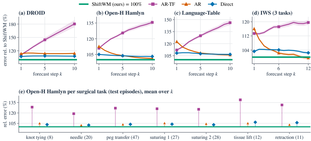
Figure 10: Error of each baseline relative to SHIFTWM (SHIFTWM=100%; above the green line: SHIFTWM better) on held-out test data. (a–d) Per forecast step; bands: paired 95% bootstrap (sessions for DROID, episodes elsewhere); IWS weights its three tasks equally. (e) Per Open-H surgical task, mean over k (number of test episodes in brackets).
