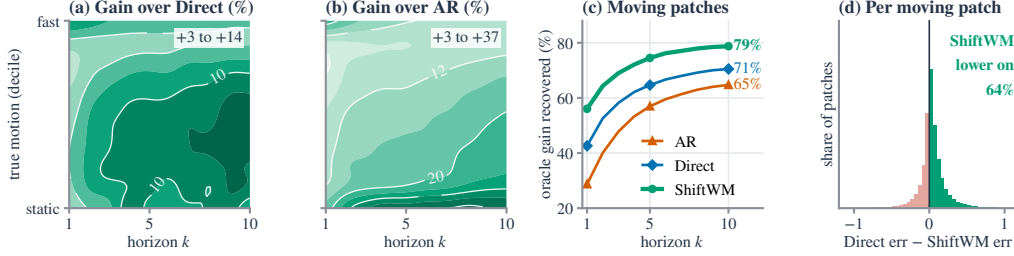
Figure 13: Where the gains lie (held-out DROID). (a,b) Error reduction of SHIFTWM per horizon and decile of true patch change (%). (c) Share of the oracle-move gain recovered on moving patches. (d) Per-patch error difference to Direct at k=10 on moving patches (green: SHIFTWM lower).
