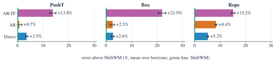
Figure 6: IWS per task: error of each baseline above SHIFTWM (200 official handles per task, mean over k , seed 0; paired 95% CIs).
