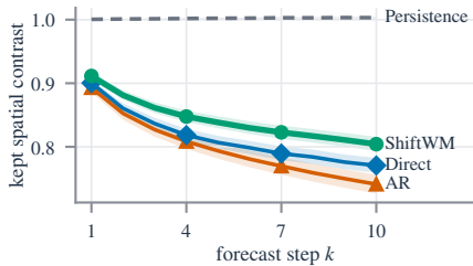
(c) Forecasts stay sharp
