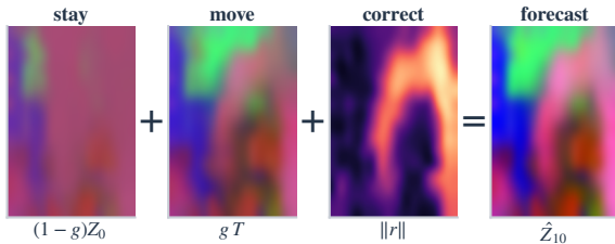
(b) How ShiftWM composes a forecast
