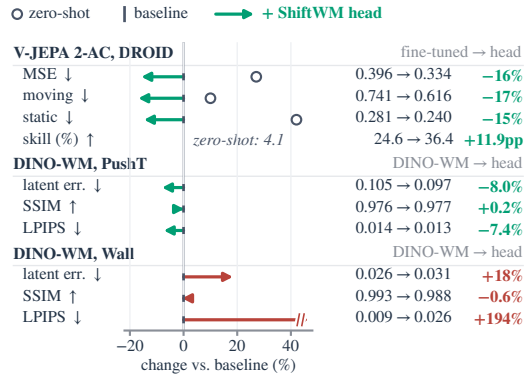
Figure 4: SHIFTWM as a plug-in head: change from adding the head to the same model (same data, schedule, loss). V-JEPA 2-AC: DROID test, base = fine-tuned (2 seeds), circles = zero-shot; DINO-WM: validation. Green better, red worse; numbers in Table 2.
