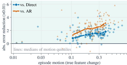
(b) and its absolute gain grows with motion
