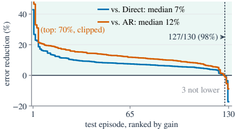
(a) ShiftWM has lower error on almost every episode
