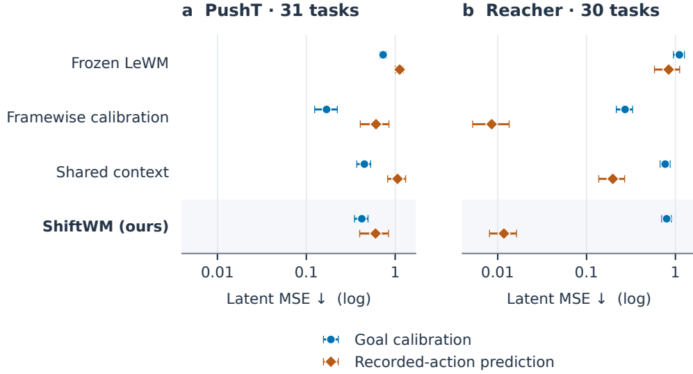
Figure 20: Prediction and goal calibration are distinct errors. Posthoc development diagnostics for frozen LeWM and three seed-0 trained models. Both errors are per-dimension MSE in fixed pre-trained coordinates against the same canonical goal; lower is better. Blue circles denote goal calibration; orange diamonds use the five recorded future action blocks. Horizontal axes are logarithmic so small errors remain visible. Error bars are 95% trajectory-seed bootstrap intervals, excluding common support-only successes; they do not measure training-seed variation. Small recorded-action prediction error alone does not establish accurate goal calibration or successful planning.
