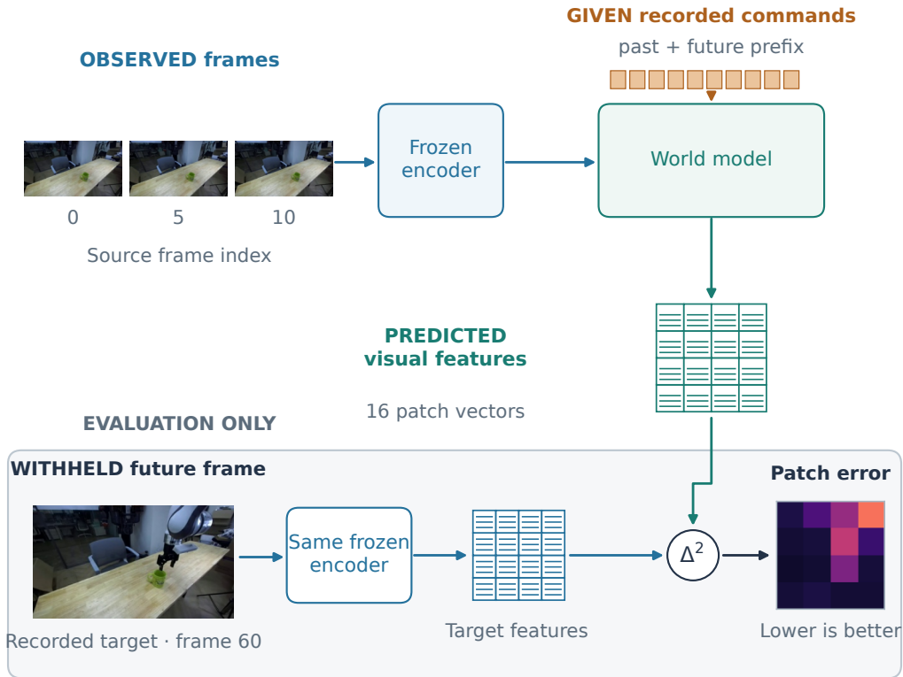
Figure 23: The recorded-video prediction task. The model receives three observed images and recorded robot commands, then forecasts visual-feature vectors for a future time. The withheld future RGB frame is used only for evaluation: the same frozen DINO encoder supplies its target features, which are compared with the forecast. The model outputs features, not a generated RGB frame or a chosen robot action. The 16 vector glyphs denote feature vectors schematically; the final heatmap is the actual three-seed h = 10 per-patch standardized feature error for the prespecified median episode’s first window (mean MSE 0.1727; one shared scale 0–0.787 across the companion gallery). Bright patches have larger feature error; this is not a pixel-reconstruction error map. The example’s episode-average gain is +5.358%, but this fixed displayed window has a -0.305% gain against the autoregressive baseline. Recorded images are unchanged DROID observations (CC BY 4.0); the target frame never enters the forecasting model.
