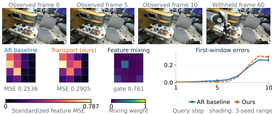
Figure 25: Recorded-video examples and spatial feature errors. Best, median and worst cases use prespecified three-seed episode-level native h10 gain versus the matched 4 \times 4 autoregressive baseline. The first eligible window is always shown: the median episode gains +5.358%, but its displayed window regresses by -0.305%. Withheld future frames enter only the evaluator. Images: DROID (CC BY 4.0). Error maps average squared standardized errors over 384 channels and three seeds, with one unclipped scale for all six maps. Curves show mean error and three-seed ranges (not confidence intervals): baseline, solid circles; ours, dashed diamonds. Mixing grids show actual h10 anchor-source weights for target cell (row 2, column 2), averaged across seeds; gates appear below. These are semantic feature mixtures, not physical flow or causal attribution. Population counts and episode- and seed-averaged native-grid endpoint gain appear above. This gain-conditioned validation gallery is not an independent test.
