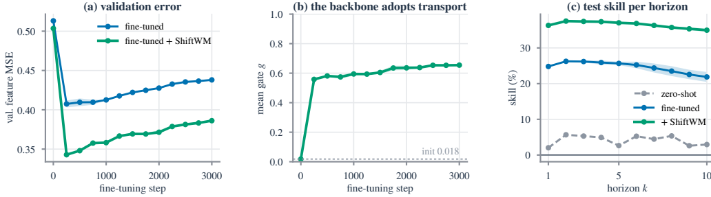
Figure 9: V-JEPA 2-AC with and without the SHIFWWM head (DROID) . (a) Validation error while fine-tuning (2 seeds). (b) Mean gate. (c) Test skill per horizon.
