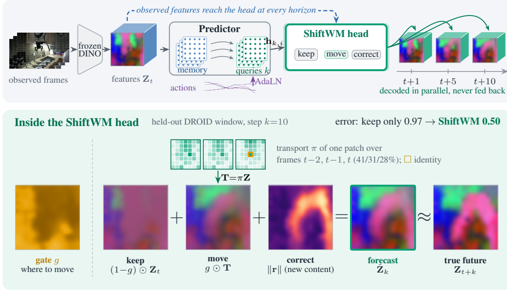
Figure 2: SHIFTWM architecture. Top: an action-conditioned predictor produces one query per patch and step; observed features reach the head directly. Bottom: on a held-out window, the forecast is the sum of kept, moved and corrected observed features.
