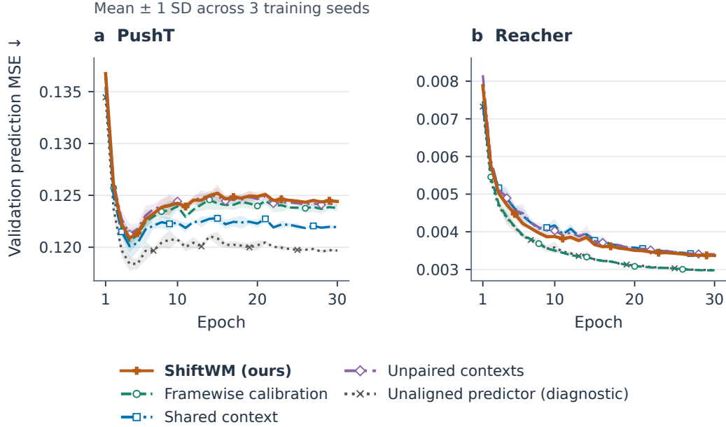
Figure 15: Validation prediction loss over the completed training campaign. Curves and shaded bands show means and sample standard deviations over three training seeds at common logged epochs. Colors and line styles identify model variants. No future epochs are extrapolated, and bands are not confidence intervals. The two panels have separate vertical scales. These are validation records, not test-set or planning-performance results.
