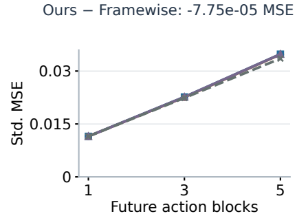
Figure 11: Real DROID recordings with measured feature-forecast errors. The primary held-out camera-1 population is summarized above three deterministically selected episodes: the largest reduction, the largest regression, and an episode nearest the median in ours-minus-Framewise h5 standardized MSE (ties by episode ID). Each image pair shows the last observed support frame and final recorded query target from the first evaluated window; these are actual photographs, not decoded predictions. Each curve averages all evaluated windows of that episode, then all three training seeds, at the three measured horizons. Panel y-axis ranges differ; methods within each panel share the same axes. Curves show point means; the full-test paired 95% h5 MSE-difference interval includes zero. The models observe three support frames and recorded commands; persistence repeats the last support feature and requires no training. The displayed images illustrate a recording and do not localize the aggregate error or establish why a method wins. Selection is outcome-conditioned and is not a frequency estimate: all-test counts and mean reduction are reported above. Error reductions are feature-forecast differences, not robot-control success or evidence of an identified causal mechanism.
