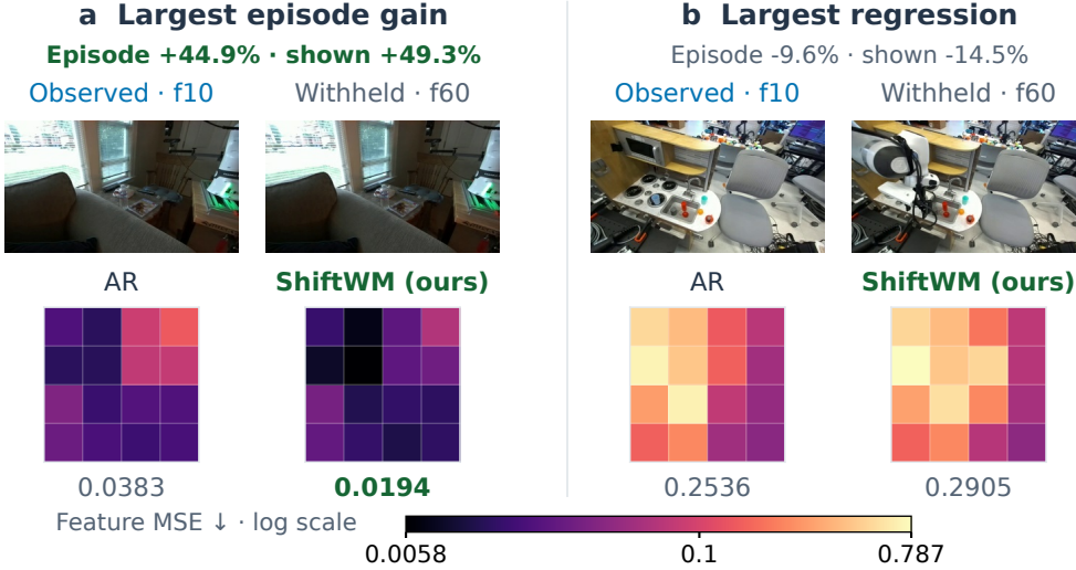
Figure 4: Selected improvement and regression on recorded video. The prespecified largest episode gain and largest regression among 141 DROID development episodes each show their first eligible window. The RGB images are recorded observations and withheld targets. AR denotes matched autoregression; ShiftWM (ours) uses bounded spatial mixing. Maps and numbers show native standardized h = 10 feature MSE over three seeds, with one unclipped logarithmic scale shared across all six original gallery maps. Positive gains mean lower error; episode and shown-window averages differ. The appendix retains the median case and full selection record. Images: DROID (CC BY 4.0).
