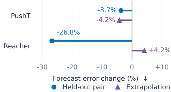
Figure 18: Separating what is seen from how the world responds. Left: a generated concept illustration distinguishes appearance from dynamics; it is not simulator output. Evaluated appearance changes are pointwise RGB transforms, not camera-viewpoint changes. Right: relative forecast MSE@5 change of ShiftWM (ours) versus Framewise calibration, computed from the ratio of three-training-seed means. Negative values indicate lower error. Gains on held-out pairs do not extend to Reacher extrapolation. These point summaries are not planning results or significance estimates; Figure 17 reports raw errors, all aligned controls, and seed variability.
