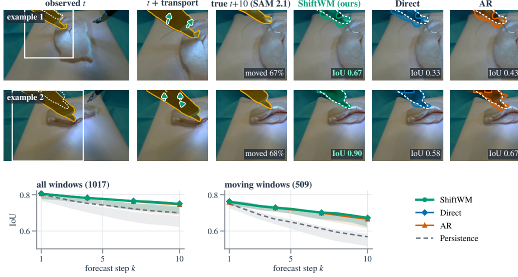
Figure 16: Segmentation view, Hamlyn (target: instruments; 1017 windows, 140 episodes). Examples: the two moving windows (distinct episodes) with the largest k=10 IoU advantage of SHIFTWm over the better baseline, SHIFTWm IoU \geq 0.5 ; illustrative, averages in Table 17. Columns as in Figure 14.
