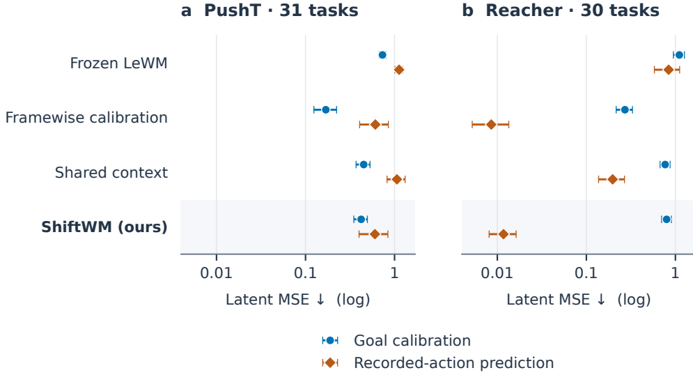
Figure 19: Prediction and goal calibration are distinct errors. Posthoc development diagnostics for frozen LeWM and three seed-0 trained models. Both errors are per-dimension MSE in fixed pre-trained coordinates against the same canonical goal; lower is better. Blue circles denote goal calibration; orange diamonds use the five recorded future action blocks. Horizontal axes are logarithmic so small errors remain visible. Error bars are 95% trajectory-seed bootstrap intervals, excluding common support-only successes; they do not measure training-seed variation. Small recorded-action prediction error alone does not establish accurate goal calibration or successful planning.
