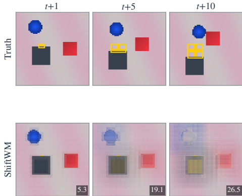
(a) forecasts (MSE \times 10^{-3} in corner)
