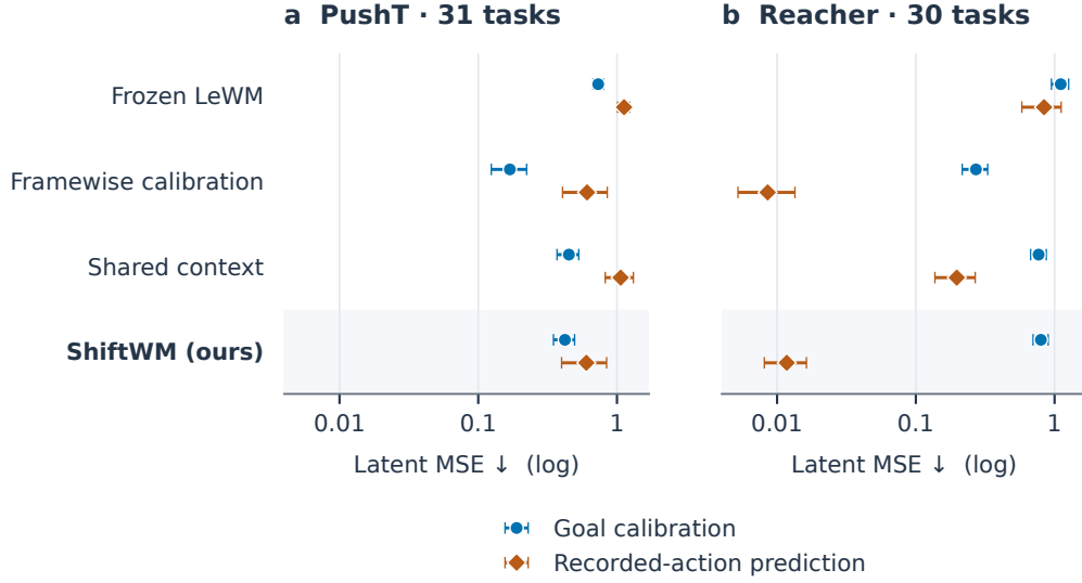
Figure 15: Prediction and goal calibration are distinct errors. Posthoc development diagnostics for frozen LeWM and three seed-0 trained models. Both errors are per-dimension MSE in fixed pre-trained coordinates against the same canonical goal; lower is better. Blue circles denote goal calibration; orange diamonds use the five recorded future action blocks. Horizontal axes are logarithmic so small errors remain visible. Error bars are 95% trajectory-seed bootstrap intervals, excluding common support-only successes; they do not measure training-seed variation. Small recorded-action prediction error alone does not establish accurate goal calibration or successful planning.
