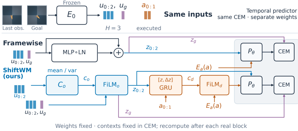
Figure 15: What changes in the computation. Both methods use the same frozen encoder, predictor architecture, history/action interface and CEM, with separately trained predictor weights. Framewise applies a per-image residual MLP; ShiftWM (ours) adds observation and dynamics contexts. The goal is calibrated but never enters context inference. GRU inputs are [z_i, z_{i+1} - z_i, \tilde{a}_i] ; E_a(a) embeds executed past and candidate future actions. This code-derived schematic describes operations and does not establish component causality.
