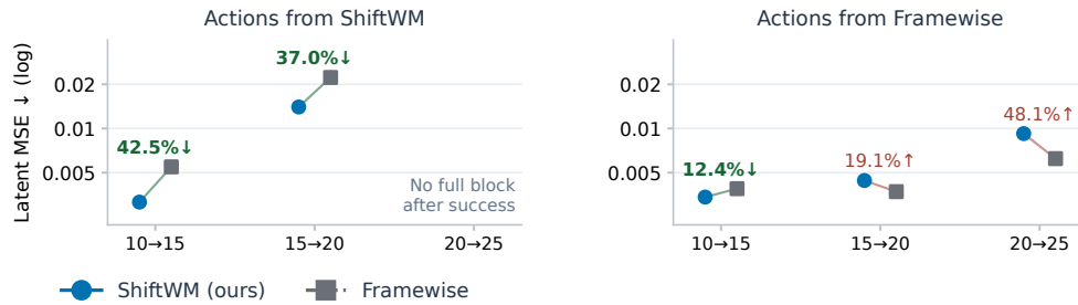
Figure 21: Reacher: two accurate forecasts accompany coordinated success. Episode 2031004. A: observed poses use a common crop and goal outline. B: both unwrapped joint errors fall below 0.05 radians at call 23 for ShiftWM (ours); Frame-wise fails at call 50. A smaller error in one joint at an earlier time does not satisfy the joint criterion. C: ShiftWM's next-observation MSE is 42.5% and 37.0% lower on the two full transitions along its own execution, but lower on only one of three transitions along Frame-wise's execution. These paired measurements show a local predictive advantage, without establishing component causality or average planning gains.
