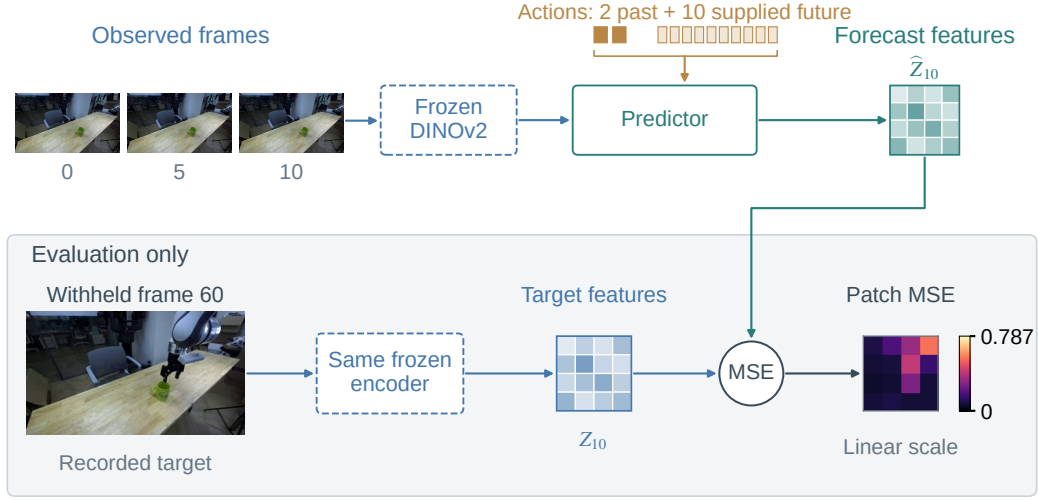
Figure 6: Available inputs and withheld evaluation targets. Three observed frames (0, 5, 10), two past action blocks and ten supplied future blocks determine the feature forecast. Frame 60 enters only the evaluator through the same frozen DINOv2 encoder. One block spans five source-frame intervals, not seconds. Tiles are schematic feature grids; the heatmap is the actual three-seed standardized h = 10 patch error for the prespecified median-by-episode-gain case’s first window (MSE 0.1727; gain -0.305\% versus autoregression). Its linear scale retains the original 0–0.787 range. Recorded DROID images are unchanged (CC BY 4.0); no RGB or robot actions are generated.
