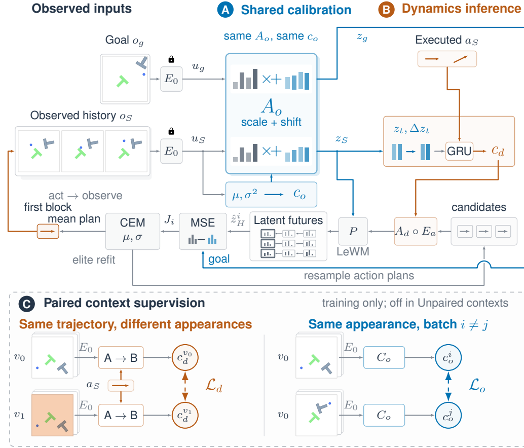
Figure 13: ShiftWM (ours): separate contexts with paired supervision. A infers observation context from past-feature statistics and shares one calibration map between history and goal. B infers dynamics context from corrected transitions and executed actions, then conditions action embeddings in the reused LeWM predictor. C adds offline penalties: \mathcal{L}_d compares different appearances of the same trajectory and actions, each through its own A–B computation; \mathcal{L}_o compares distinct batch entries with the same appearance. Dashed links denote penalties, not guaranteed equal or identified contexts. Training frames in C represent support clips; the upper frames illustrate deployment inputs. The encoder is frozen; contexts, adapters, and reused prediction modules train offline. Online, weights and contexts stay fixed within CEM search. Each candidate action sequence produces a latent rollout, scored by terminal MSE to the calibrated goal. CEM refits its action distribution to low-cost elites; the controller executes the first block of the final mean plan and replans. Feature glyphs and the rollout/cost example are schematic, not measurements. Canonical query losses and the exact planning budget are given in the text.
