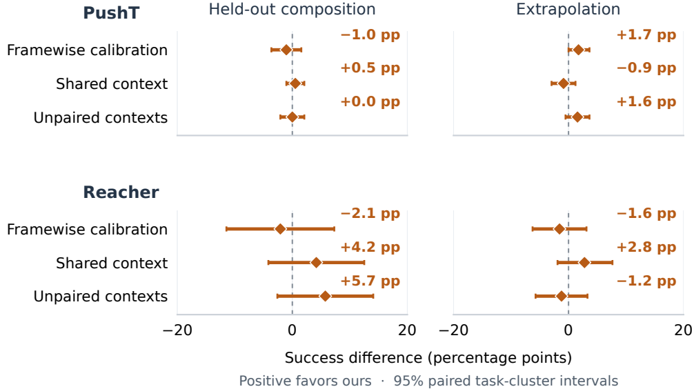
Figure 27: Paired planning differences. Points show mean paired raw success differences across three training seeds; positive values favor ShiftWM (ours). Bars are 95% initial-state-cluster bootstrap intervals conditional on those trained models, not training-seed standard deviations or uncertainty over the training population. Pending comparisons have no point estimate. These exploratory intervals are not multiplicity-adjusted.
