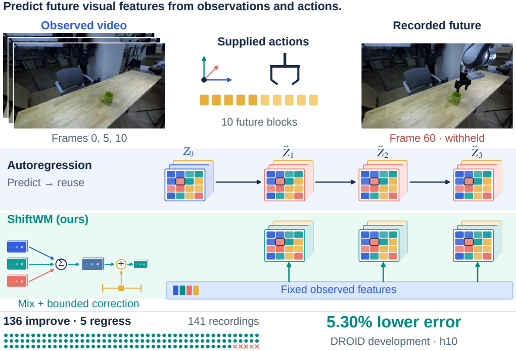
Figure 1: Predict visual change without replacing the observed reference. Top: unchanged DROID images illustrate the prespecified median case; the future frame is an evaluator target, not predicted RGB. Middle: autoregression feeds forecasts forward; ShiftWM mixes the fixed observed feature grid and adds bounded corrections. Both paths use the same available history and actions. Feature layers, commands and the mixing inset are schematic; three drawn forecast steps illustrate a dependency that continues to the ten-step endpoint. Bottom: one mark per development episode reports lower (circle) or higher (cross) native ten-step feature error versus matched autoregression, averaged over windows and three seeds. The 5.30% reduction uses population mean errors, not mean episode percentages. Figure 3 reports uncertainty; Figure 4 gives the matched case-level comparisons. Images: DROID (CC BY 4.0).
