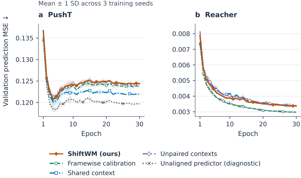
Figure 16: Validation prediction loss over the completed training campaign. Curves and shaded bands show means and sample standard deviations over three training seeds at common logged epochs. Colors and line styles identify model variants. No future epochs are extrapolated, and bands are not confidence intervals. The two panels have separate vertical scales. These are validation records, not test-set or planning-performance results.
