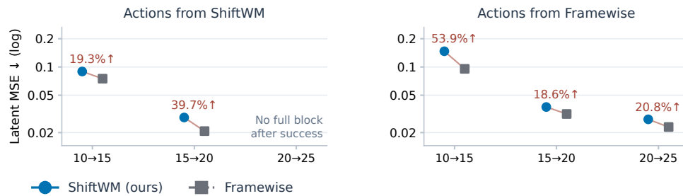
Figure 20: PushT: success does not require winning every diagnostic. Episode 2031024. A: real observations and a display-only goal outline. The green T is an unscored renderer marker; dashed contours show the task goal. B: at call 20, ShiftWM (ours) has approximately half the remaining combined position error, while Framewise has the smaller angle error. ShiftWM meets both tolerances at call 21; Framewise moves away and fails at call 50. C: each pair tests two models on the same realized transition, grouped by the behavior policy. ShiftWM has higher one-block prediction error on all five pairs despite its successful execution. The conditional diagnostic therefore rejects a uniform prediction-improvement explanation for this case.
