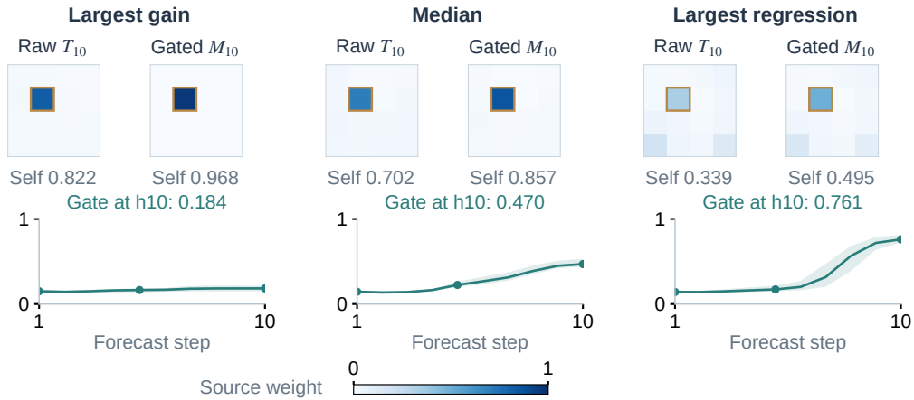
Figure 7: Measured mixing and gate behavior for the same three cases. At the prespecified target patch (row 2, column 2), the first map shows the learned source weights T_{10}[j, :] and the second shows the effective anchored weights M_{10}[j, :] , where M_h = (1 - g_h)I + g_h T_h rowwise. The outline marks the source at the target’s own location; values underneath give its weight. Maps use one linear [0, 1] scale and average three seeds after applying the gate within each seed. Curves show the target patch’s gate mean and seed range, not confidence intervals. These are measured feature mixtures, not physical motion or causal explanations of the error differences in Figure 4.
