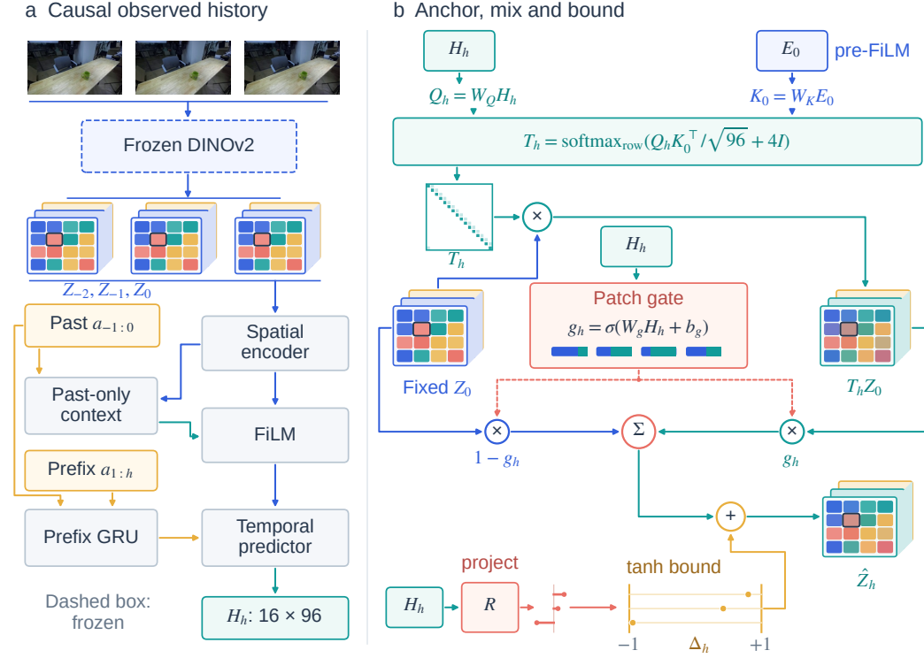
Figure 2: ShiftWM (ours): observed features remain the source of every forecast. (a) Frozen DINOv2 features are pooled to 4 \times 4 and normalized using fixed training-only channel statistics. Trainable spatial encoding feeds a past-only patch-mean context and FiLM. A separate chronological action GRU supplies the two past states and the prefix endpoint at h to the trained LeWM temporal architecture. (b) Every H_h port denotes the same horizon state. Keys use the fixed last-observed spatial encoding E_0 before FiLM; the source Z_0 is instead the last observed normalized 16 \times 384 feature grid. Dashed coral control paths apply complementary per-patch weights to the two feature branches. Row-stochastic mixing and this sigmoid gate form (1 - g_h)Z_0 + g_h T_h Z_0 . The distinct innovation branch applies R = \text{LayerNorm} + \text{Linear}_{96 \rightarrow 384} and \Delta_h = \tanh R(H_h) , then adds it to the blend. The unit bound applies in normalized coordinates; inverse normalization is omitted. Only DINOv2 weights are frozen. Colored feature objects, gate bars and saturation examples are schematic; DROID observations are unchanged (CC BY 4.0). No future RGB enters the model. Appendix A gives the full protocol.
