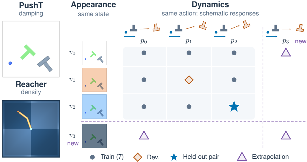
Figure 14: Composition protocol. Real task frames and exact RGB transforms illustrate observation changes; response glyphs are schematic. PushT varies damping and Reacher varies density. Seven pairs train the model, (v_1, p_1) is development, and (v_2, p_2) is held-out composition. Three extrapolation pairs introduce new values. Independent test trajectories cover all nine in-range pairs. Split identities precede paired rendering; factor labels are unavailable to the deployed model.
