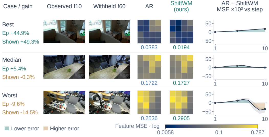
Figure 1: Prespecified best, median and worst cases. The episode-gain ranks among 141 DROID development recordings each show their first eligible window. AR denotes matched autoregression. Full RGB frames are recorded observations ( f_{10} ) and withheld targets ( f_{60} ). Maps show three-seed native, training-standardized h = 10 feature MSE on one unclipped logarithmic scale. Curves show mean paired AR-minus-ShiftWM error with common \pm 70 \times 10^{-3} MSE limits; bands show seed minima/maxima, not confidence intervals. Teal gains mean lower error; amber shows regressions. Each forecast step consumes five native commands. Episode (Ep) gains average windows; the shown median window instead regresses. Images: DROID (CC BY 4.0).
