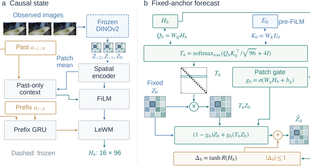
Figure 2: ShiftWM (ours): fixed spatial anchoring with bounded innovation. (a) Three frozen DINOv2 grids enter spatial encoding. Patch-mean past transitions infer context for FiLM; a chronological past-plus-query-prefix GRU supplies LeWM, without actions beyond horizon h . Learned modules after DINOv2 train offline. (b) Z_0 is the last observed 16 \times 384 grid in shared per-channel training-normalized coordinates; E_0 is its spatial encoding before FiLM. Both H_h labels denote the same horizon state. The fixed 4 \times 4 anchor is mixed by a 16 \times 16 row-stochastic matrix; a per-patch sigmoid gate blends it, and the projected innovation \Delta_h = \tanh R(H_h) is bounded elementwise by one. Here R is layer normalization followed by an affine projection. Grids and weights are schematic; DROID images are unchanged observations (CC BY 4.0). Outputs are features, not RGB; Appendix A gives details.
