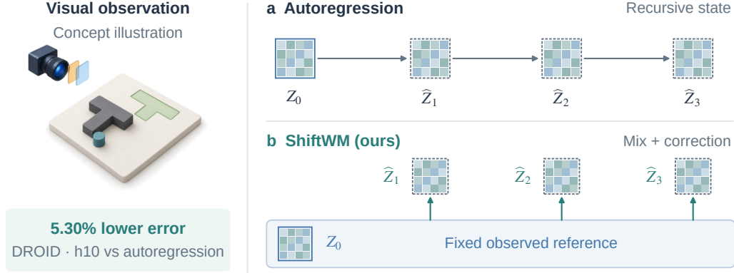
Figure 1: Forecast change while retaining the observed reference. Autoregression passes predicted features into the next step. ShiftWM (ours) draws every horizon’s mixture from the same observed grid and adds a bounded correction. Supplied actions condition both paths; Figure 2 gives the full computation. The scene and feature tiles are conceptual. The measured callout is the native ten-step endpoint feature-error reduction against matched autoregression on three-seed DROID development data.
