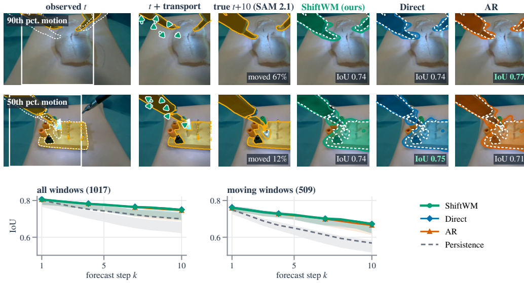
Figure 16: Segmentation view, Hamlyn (target: instruments; 1017 windows, 140 episodes). Rows: the QC-passing windows at the 90th and 50th percentile of motion. Columns as in Figure 14.
