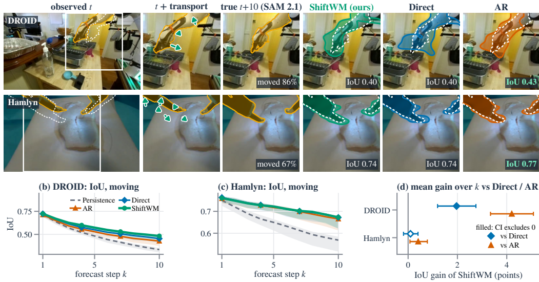
Figure 14: Where does the arm go? (a) Held-out windows at the 90th percentile of motion (fixed rule): SAM 2.1 mask at t and t+10 (yellow; dashed white: true future), SHIFW transport arrows, and the region each k=10 forecast labels as arm/instrument (heat: soft probability; IoU in the corner). (b,c) IoU vs. horizon on moving windows (95% CIs over episodes). (d) Paired gain of SHIFW, averaged over k ; filled: CI excludes 0.
