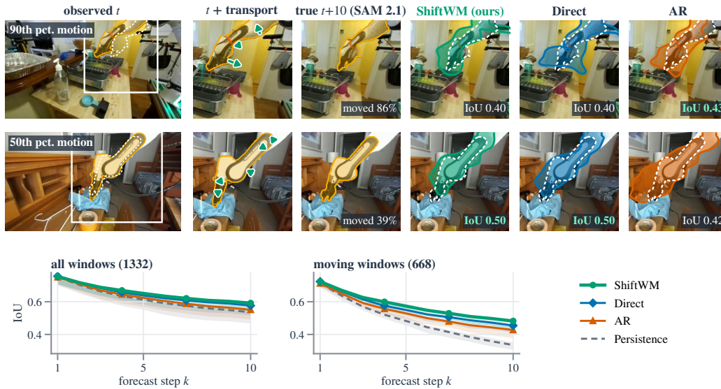
Figure 15: Segmentation view, DROID (target: robot arm; 1332 windows, 123 episodes). Rows: the QC-passing windows at the 90th and 50th percentile of motion. Columns as in Figure 14.
