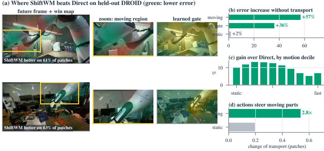
Figure 5: Where and why SHIFTWM wins (held-out DROID, k=10 ). (a) Win map (green: SHIFTWM lower error), zoom and gate. (b) Transport knockout. (c) Gain per motion decile. (d) Action steering.
