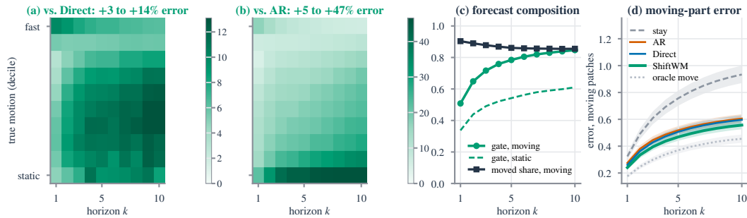
Figure 11: Anatomy of the gains (held-out DROID) . (a,b) Error reduction by horizon and motion decile. (c) Gate and share of the forecast carried by moved features. (d) Moving-part error with 95% CIs.
