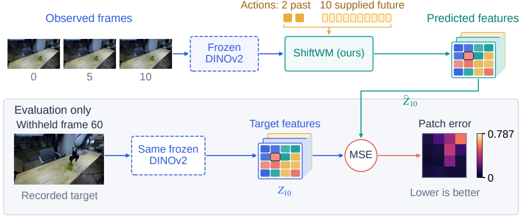
Figure 6: Recorded inputs, predicted features, withheld evaluation. Three observed frames (source indices 0, 5, 10), two past action blocks and ten supplied future blocks determine the feature forecast. Frame 60 enters only the evaluator through the same frozen DINOv2 encoder. Each block spans five source-frame intervals, not seconds. Layered feature objects are schematic; the heatmap is the actual three-seed, training-standardized h = 10 patch MSE for the prespecified median-by-episode-gain case’s first window (mean 0.1727; gain -0.305\% versus autoregression), with the unchanged linear 0–0.787 scale. Recorded DROID images are unchanged (CC BY 4.0). Neither future RGB nor robot actions are generated.
