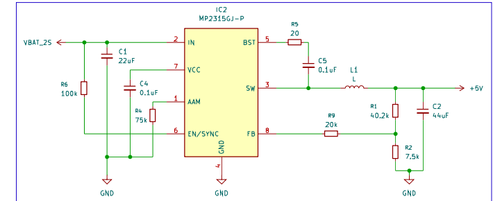
5V Battery Power for Servos
