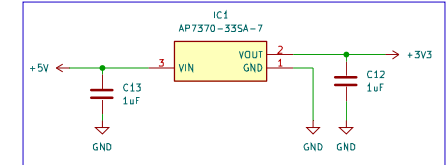
3V3 Logic Power
