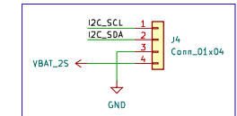
Power and Comms Port
