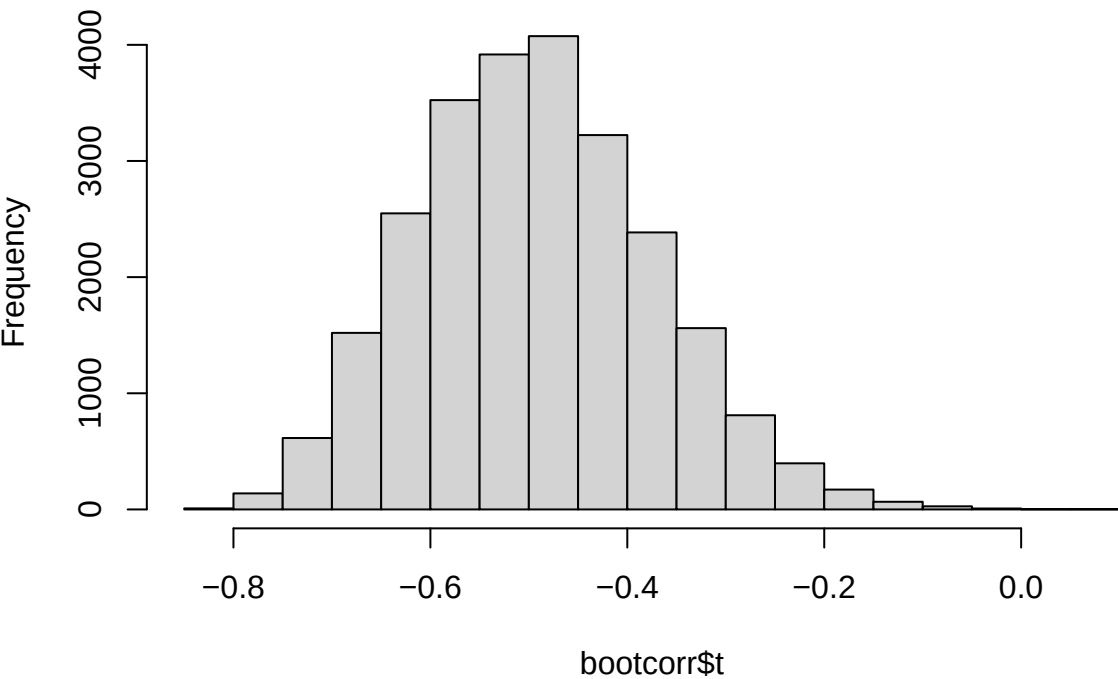
Histogram of bootcorr$t
