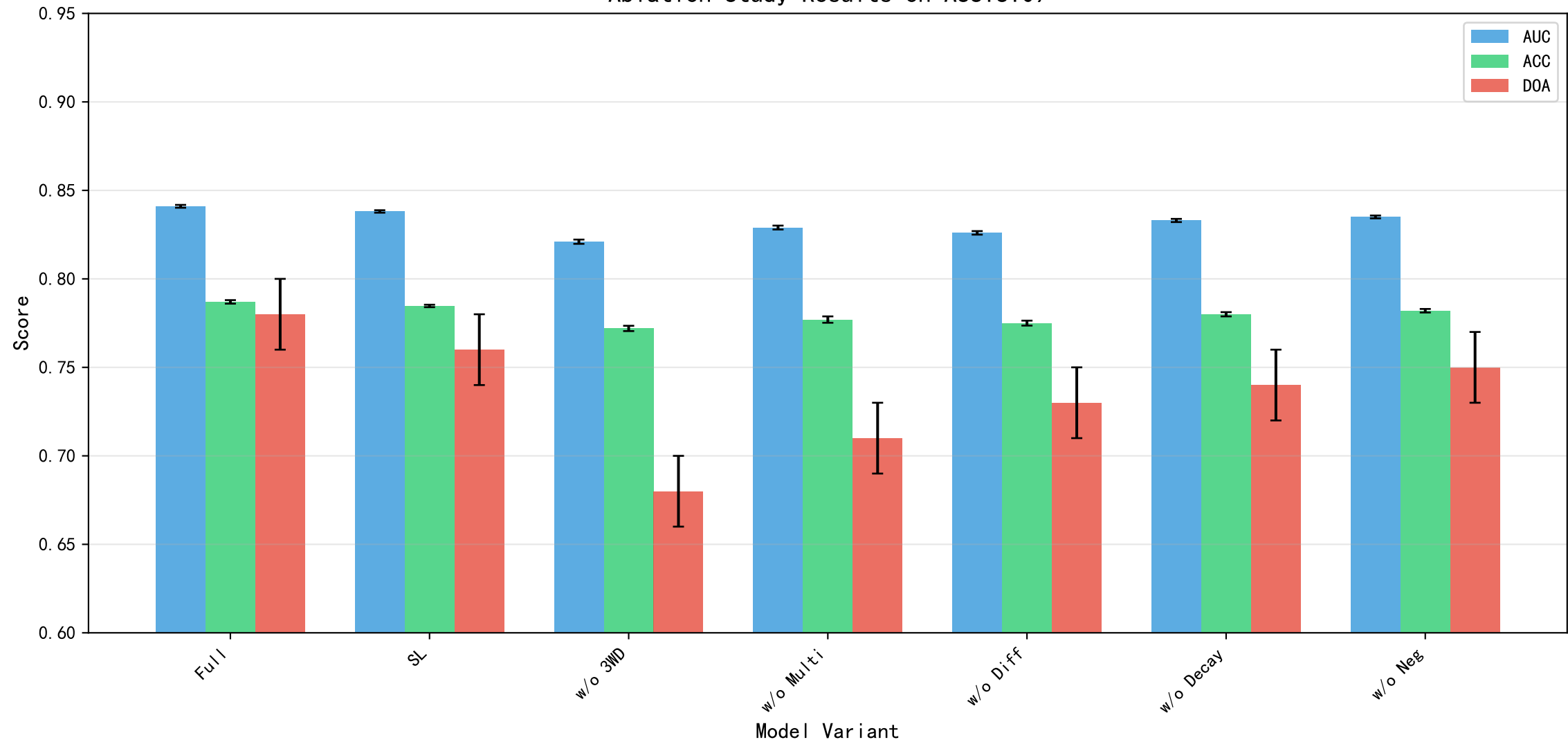
Ablation Study Results on ASSIST09
