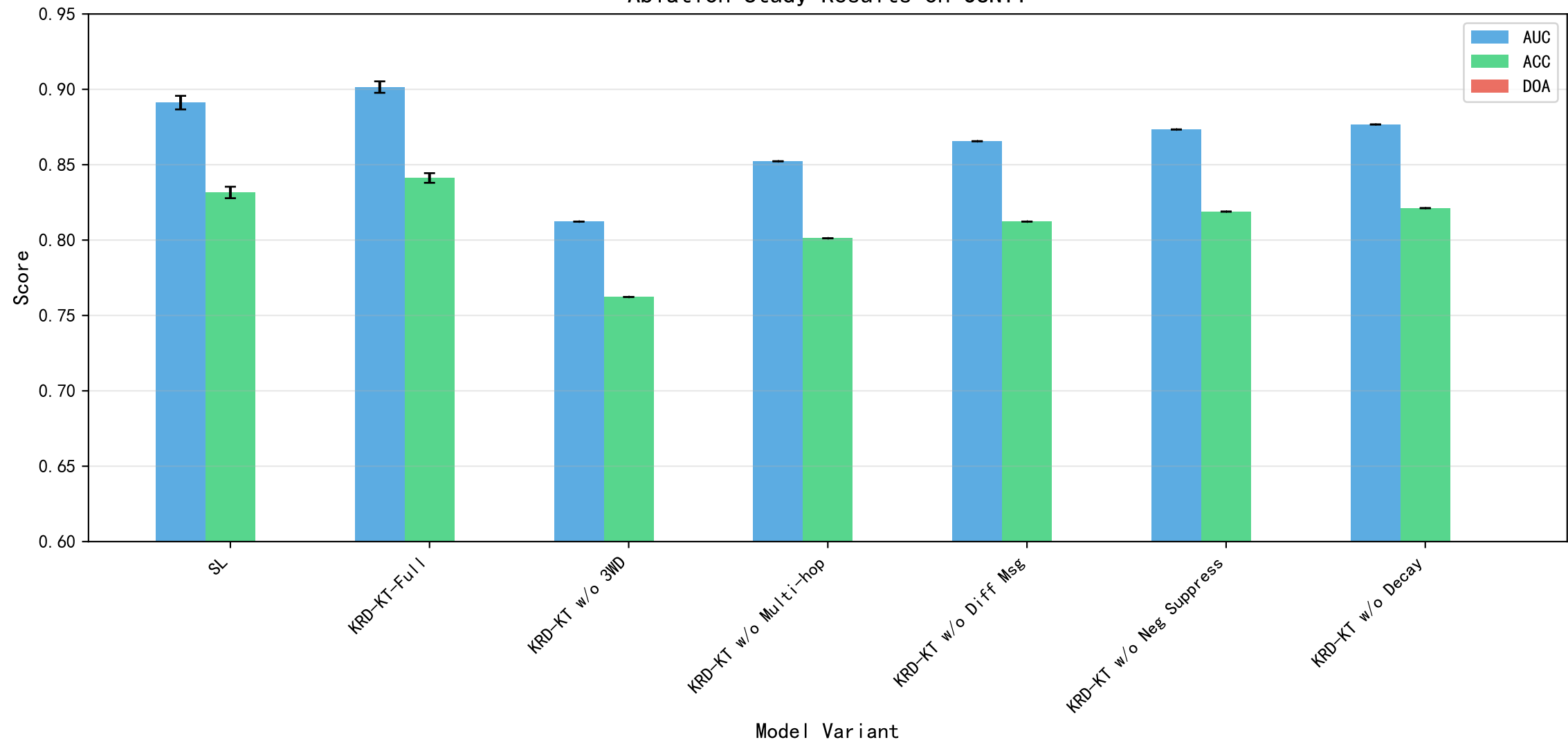
Ablation Study Results on JUNYI
