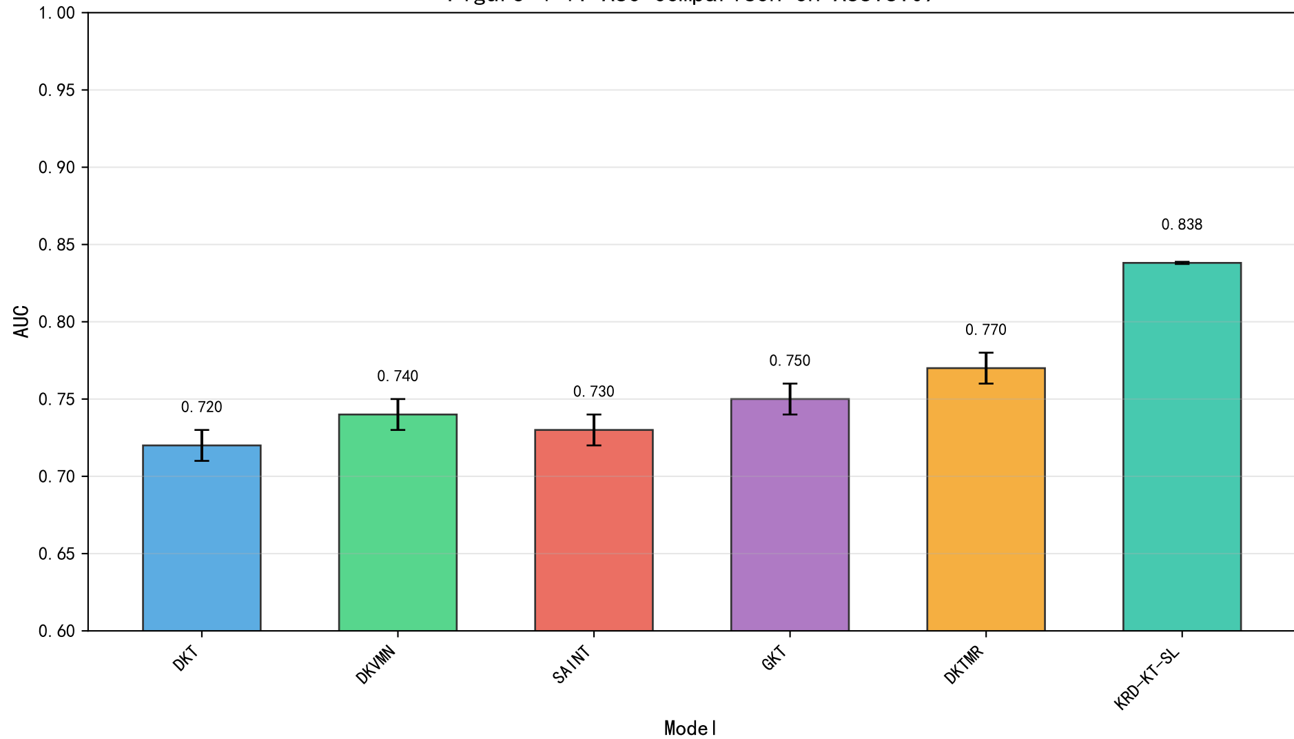
Figure 4-1: AUC Comparison on ASSIST09
