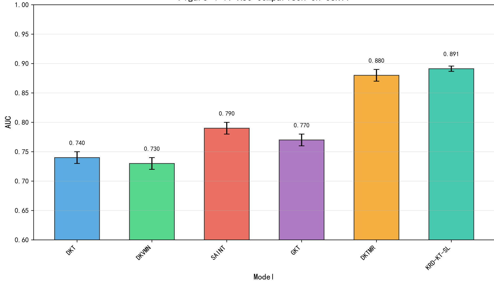
Figure 4-1: AUC Comparison on JUNYI
